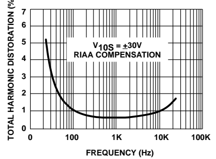
Distortion vs Frequency V_O = 1V_{\text{RMS}}
